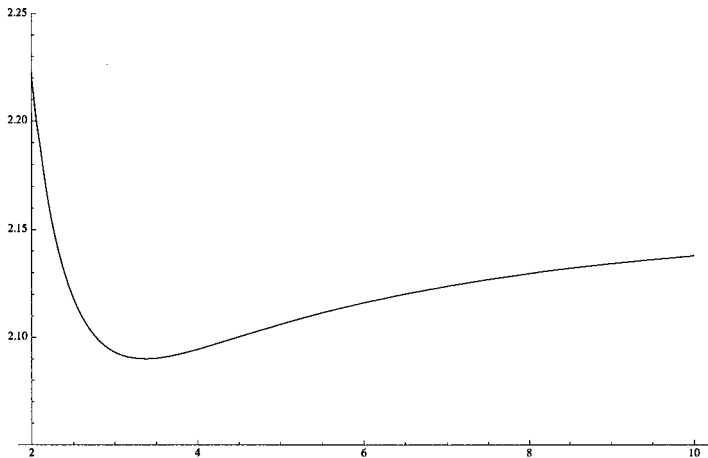
FIGURE 1. The function I on [2, 10]
